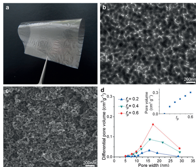
Figure 2. The structure of a bicontinuous NCF film. a) Optical photograph of an 8 × 12 cm 2 NCF film ( f_p = 0.6 ) with a thickness of 40 µm. b) TEM image of an ultrathin cross-section. The brighter regions correspond to the pores through the film. c) SEM image of an NCF film fractured after being immersed in liquid nitrogen. d) BJH pore size distributions of NCFs prepared with f_p = 0.2 , 0.4, and 0.6, respectively. Inset: pore volume of the NCF as a function of f_p .
